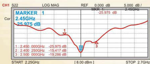
Return Loss
