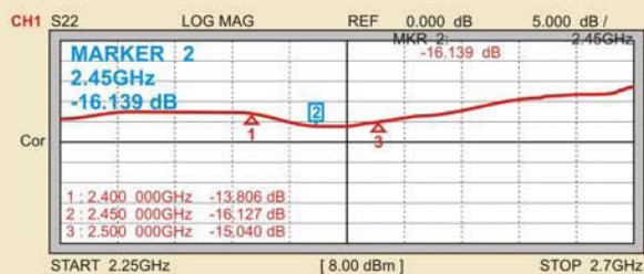
Return Loss
