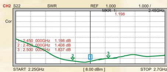
SWR
