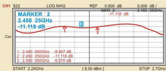
Return Loss
