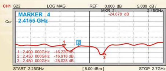
Return Loss
