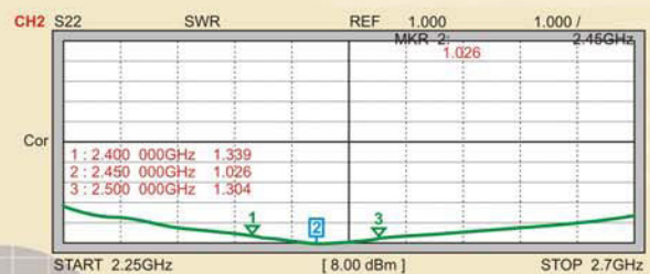
SWR
