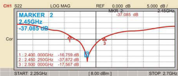
Return Loss
